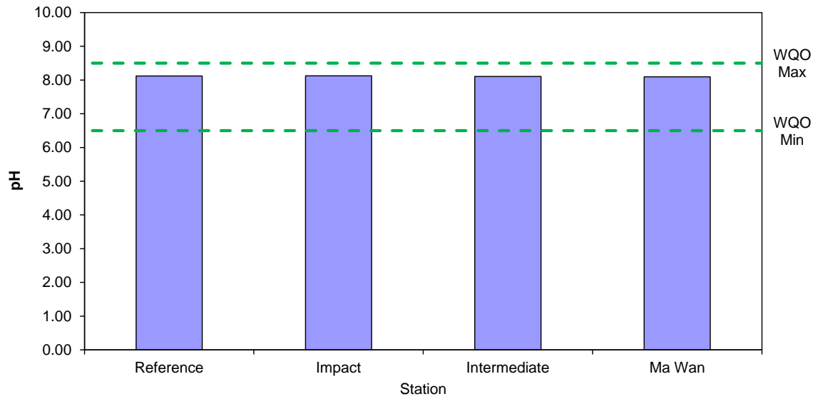
Figure 1: Level of pH recorded during Routine Water Quality Monitoring for disposal operations at ESC CMP V in November 2023
