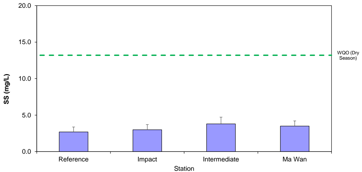
Figure 11 Concentration of Suspended Solids (SS) (mg/L; mean + SD) in water samples collected from Routine Water Quality Monitoring for disposal operations at ESC CMP V in November 2023
