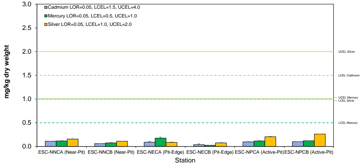
Figure 13: Concentration of Metals (Cd, Hg, Ag; mg/kg dry weight; mean + SD) in sediment samples collected from Pit Specific Sediment Chemistry Monitoring for ESC CMP Vb in November 2023
