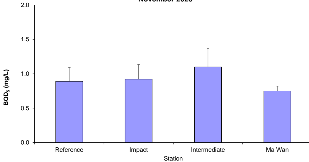
Figure 10: Level of Biochemical Oxygen Demand (BOD5) (mg/L; mean + SD) in water samples collected from Routine Water Quality Monitoring for disposal operations at ESC CMP V in November 2023
