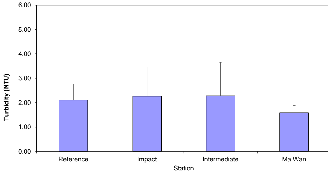
Figure 6: Level of Turbidity (NTU; mean + SD 1 ) recorded during Routine Water Quality Monitoring for disposal operations at ESC CMP V in November 2023
