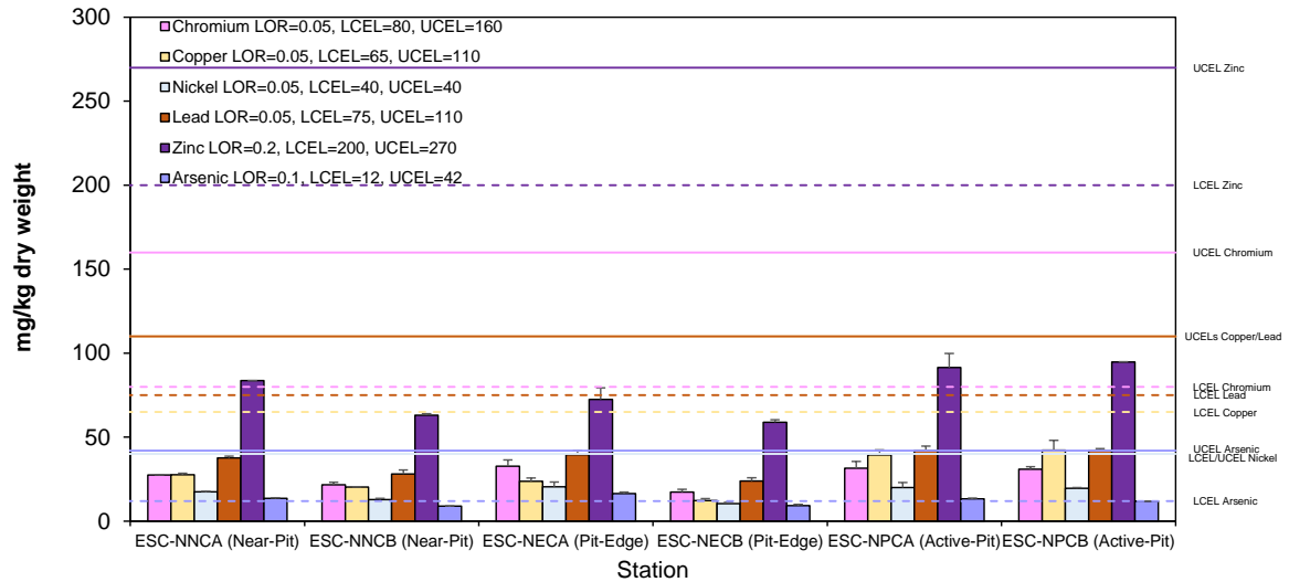
Figure 12: Concentration of Metals and Metalloid (Cr, Cu, Ni, Pb, Zn, As; mg/kg dry weight; mean + SD) in sediment samples collected from Pit Specific Sediment Chemistry Monitoring for ESC CMP Vb in November 2023
