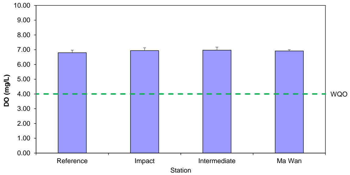
Figure 3: Concentration of Dissolved Oxygen (DO) (mg/L; mean + SD 1 ) recorded during Routine Water Quality Monitoring for disposal operations at ESC CMP V in November 2023
